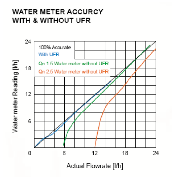
Figure 7: The Effect of the Unmeasured Flow Reducer on Water Meter Accuracy
