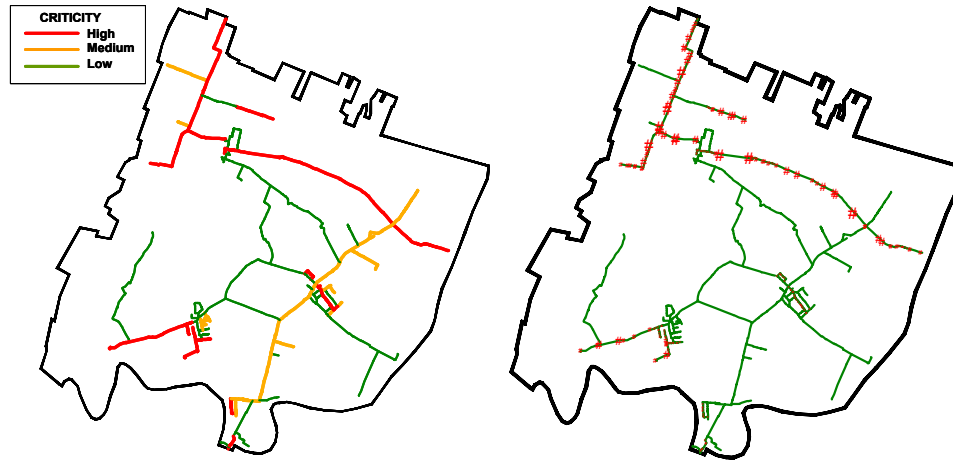
Figure 5: Pipes susceptible to leakage (left) and estimated \alpha coefficients distribution (right)
