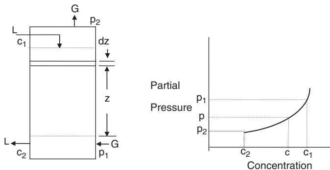
Figure 5.4 Schematic diagram of packed column.
