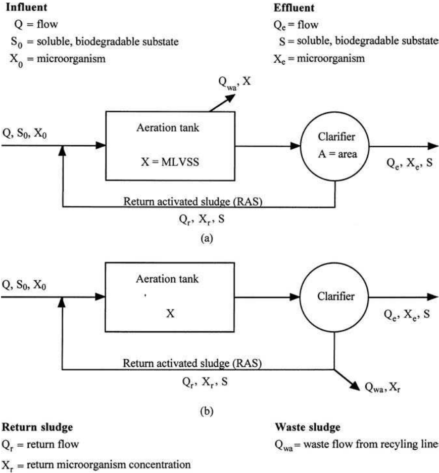
Figure 6.15 Schematic chart of complete-mix activated sludge reactor: (a) sludging wasting from the aeration tank; (b) sludge wasting from return sludge line.
