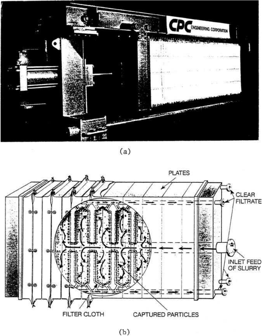
Figure 6.61 Plate and frame filter press: (a) side view of a filter press; (b) schematic cross section of chamber area during fill cycle.
