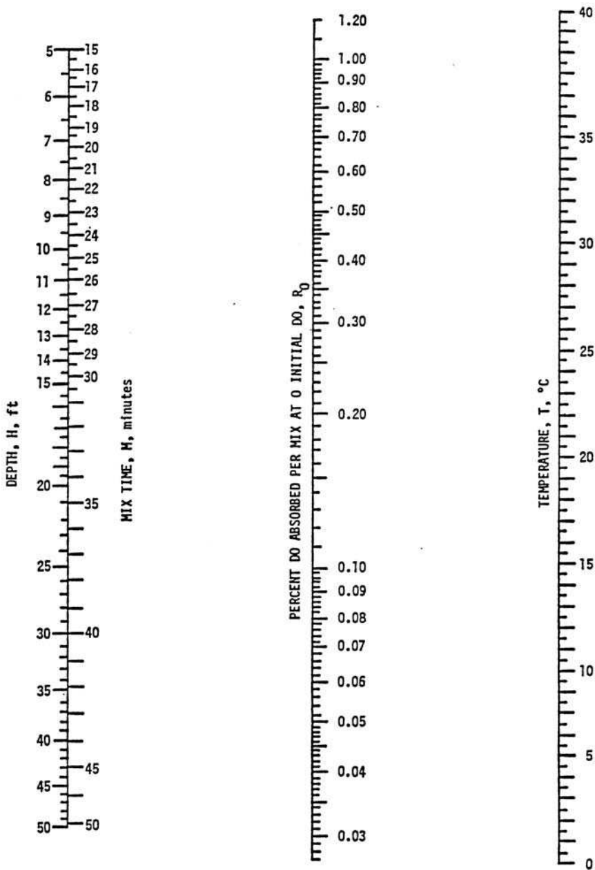
Figure 1.12 Oxygen absorption nomograph (Butts and Schnepfer, 1967).
