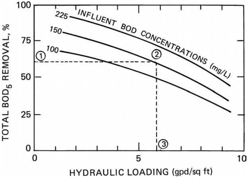
Figure 6.32 RBC process (mechanical drive) design curves for percent total BOD removal (temperature > 13°C, 55°F).
