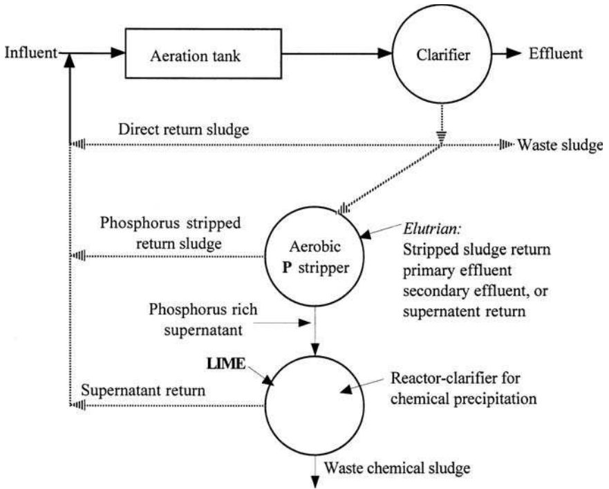
Figure 6.39 PhoStrip process.
