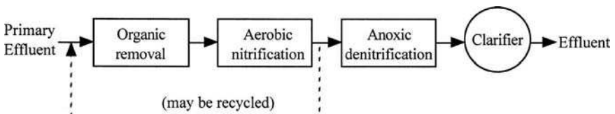
Figure 6.52 Schematic RBC process for BOD removal, nitrification, and denitrification.
