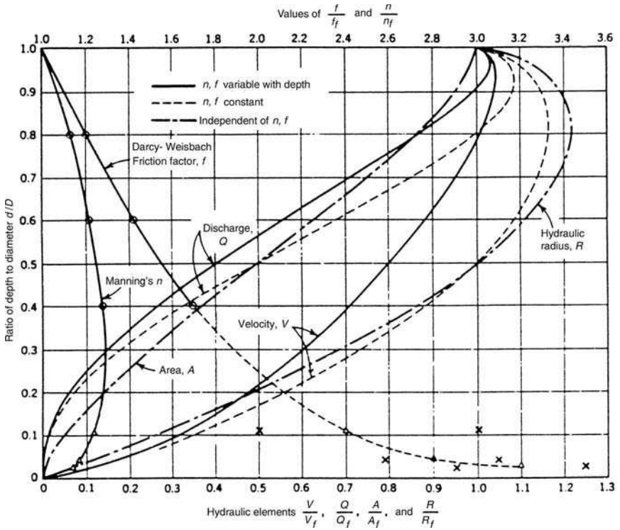
Figure 4.4 Hydraulic elements graph for circular sewers ( Metcalf and Eddy, Inc., Wastewater Engineering: Collection and Pumping of Wastewater, Copyright, 1990, McGraw-Hill, New York, reproduced with permission of McGraw-Hill ).
