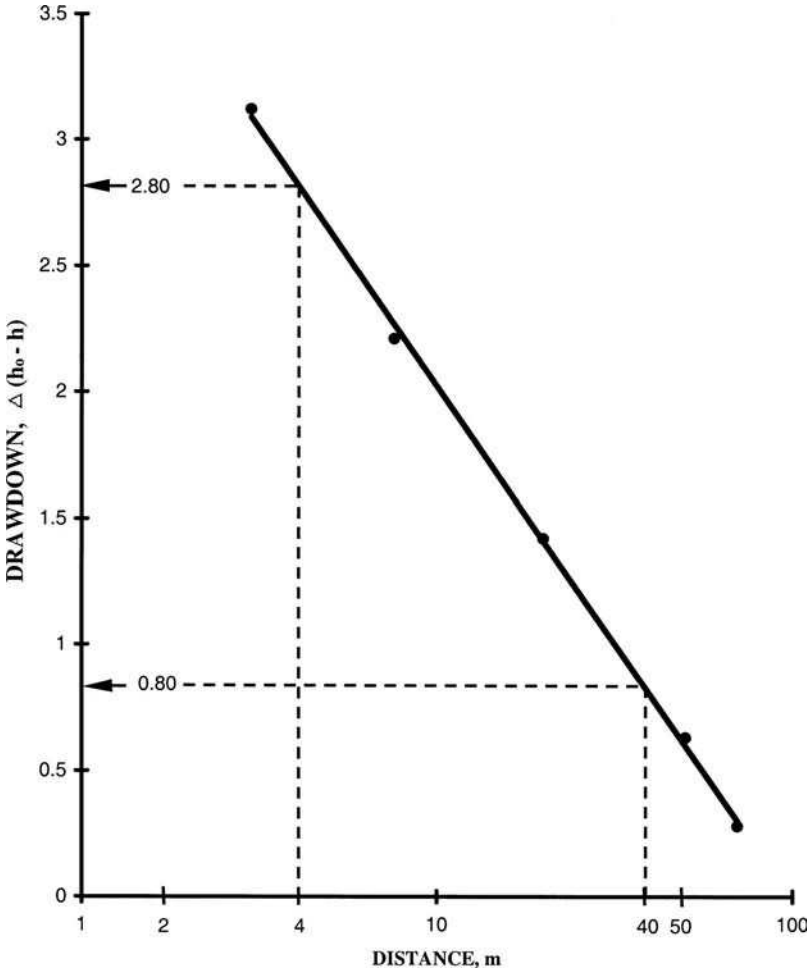
Figure 3.7 Plot of observed distance-drawdown data.
