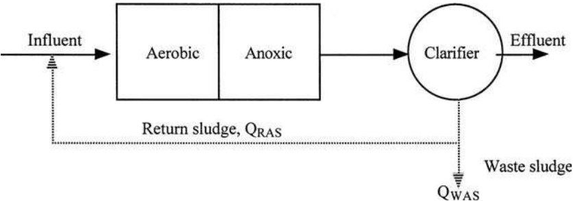
Figure 6.45 Wuhrmann process for nitrogen removal.
