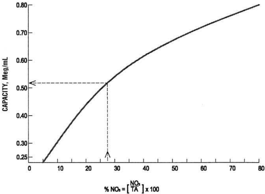
Figure 5.7 Relationship of \text{NO}_3/\text{TA} and unadjusted resin capacity for A-104 resin (US EPA, 1983).
