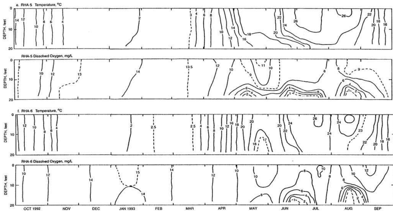
Figure 2.6 Isothermal and iso-dissolved oxygen plots for the deep stations (Lin et al. , 1996).
