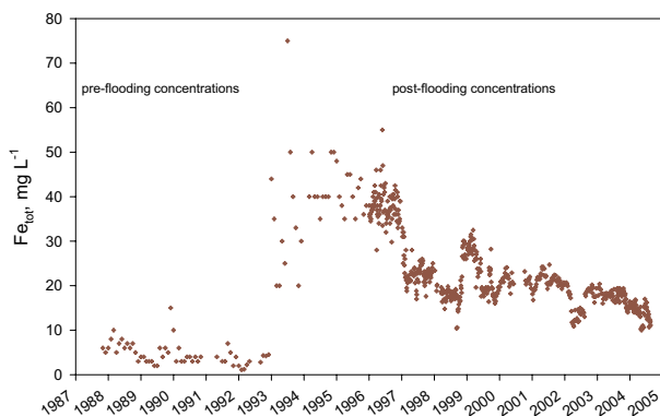
Fig. 13. Time series of changing Fe tot in the Straßberg/Germany fluorspar mine before and after the flooding of the mine in 1993 (data kindly provided by BST Mansfeld GmbH and GVV).
