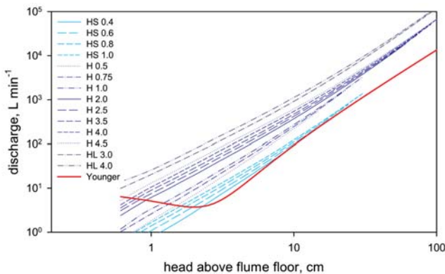
Fig. 57. Graphical comparison of the 14 different HS-, H, and HL-flume types used for flow measurements. The simplified H-flume equation of Younger et al. (2002) is given for comparison. It can only be used with heads over about 6–7 cm and for HS-type flumes.
