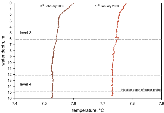
Fig. 115. Temperature–depth profile in the Felsendome Rabenstein machine shaft before and after the tracer test.
