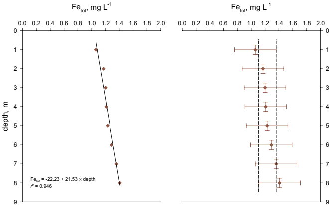
Fig. 76. Faked depth dependencies of \text{Fe}_{\text{tot}} in a waste rock pile.
