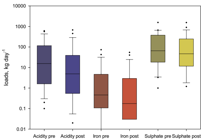
Fig. 21. Box-plot of logarithmic loads showing the mine water quality improvements in selected surface and underground mines after remining procedures were conducted; pre: pre-mining, post: post-mining situation (modified after Hawkins 1995).
