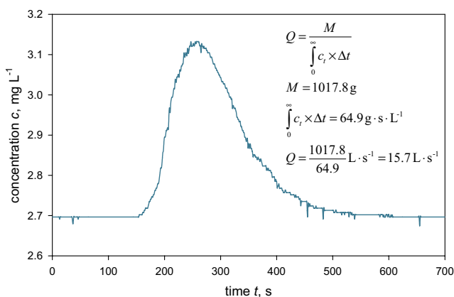
Fig. 62. Breakthrough curve and evaluation for a salt-dilution tracer test in the German Gernrode/Harz Steinbach creek. The distance between the tracer injection and the sampling site was 53 m and the complete mixing was tested in advance using a dye tracer.
