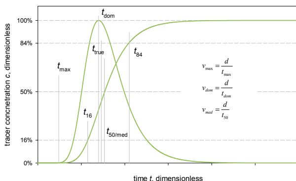
Fig. 83. Velocities that can be derived from a breakthrough curve. t_{16} and t_{84} are needed to calculate the longitudinal dispersion coefficient D_L ; t_{\text{true}} is exactly in the middle of t_{\text{dom}} and t_{\text{med}} .
