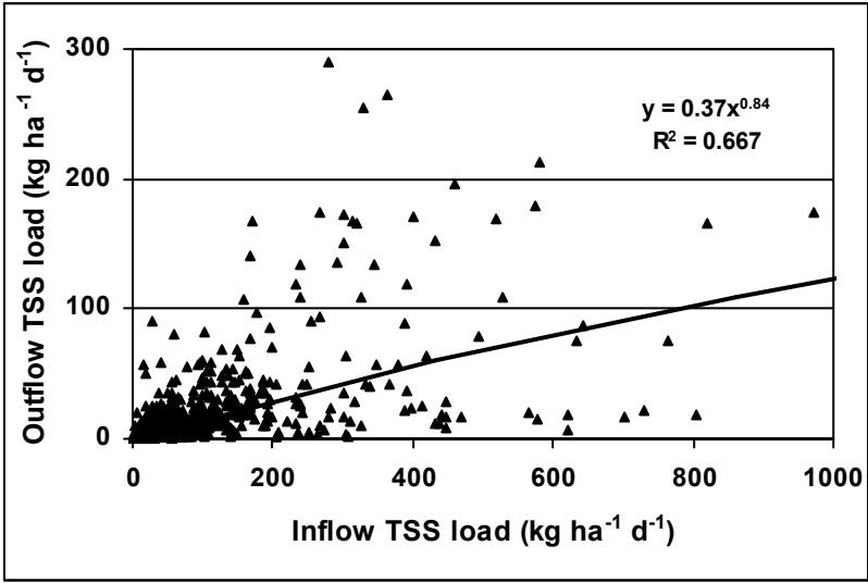
Figure 5-77. Relationship between inflow and outflow TSS loadings in HF constructed wetlands ( n=928 , inflow range 0.1 - 33,500 \text{ kg ha}^{-1} \text{ d}^{-1} ). Highest 18 values over 1000 \text{ kg ha}^{-1} \text{ d}^{-1} not shown.
