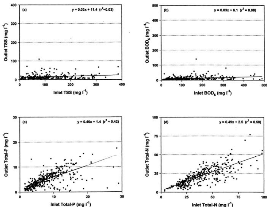
Figure 7-11. Annual mean inlet and outlet concentrations for 90 Danish HF constructed wetlands. TSS ( n=257 ), BOD 5 ( n=380 ), TP ( n=362 ), TN ( n=353 ). From Brix (1998) with permission from Backhuys Publishers.
