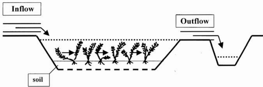
Figure 4-14. Schematic representation of a constructed wetland with submerged macrophytes. From Vymazal (2001a) with permission from Backhuys Publishers.
