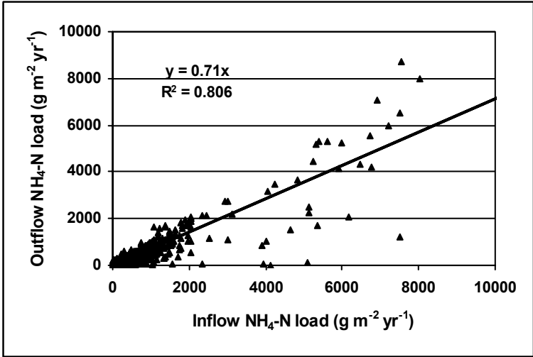
Figure 5-81. Relationship between inflow and outflow \text{NH}_4\text{-N} loads (bottom, n=827 , inflow load range 2-17,634 \text{g m}^{-2} \text{yr}^{-1} , highest 2 values not shown) in HF constructed wetlands.
