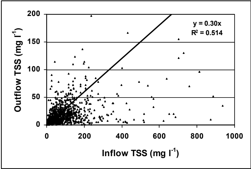
Figure 5-76. Relationship between inflow and outflow TSS concentrations in HF constructed wetlands ( n=1,022 , maximum inflow value 4,200 \text{ mg l}^{-1} , highest 17 values not shown).
