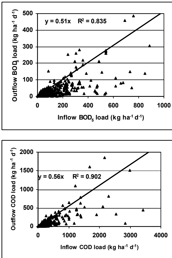
Figure 5-73. Relationship between inflow and outflow BOD 5 (top, n=988 , inflow range. 0.3 – 8,580 kg ha -1 d -1 ) and COD (bottom, n=579 , inflow range 3.3 – 14,769 kg ha -1 d -1 ) loadings in HF constructed wetlands. Highest 12 values in both charts are not shown.
