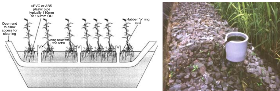
Figure 5-25. Riser pipe distribution. Left: general layout, with permission from Backhuys Publishers, right: detail of the slide collar with a vee-notch, HF Moreton Morrell. Photo by Jan Vymazal.
