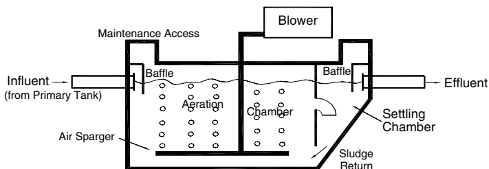
Figure 4.5 Aeration in an ATU by air spargers.
