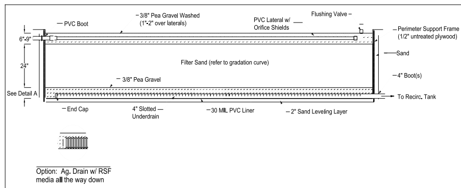
Figure 3.4 Profile view of a recirculating filter system
