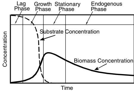
Figure 4.1 Kinetics of aerobic digestion.
