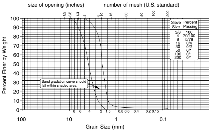
Figure 3.11 Grain size distribution chart for recirculating filter media.
