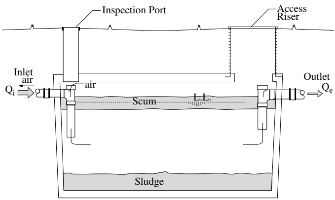
Figure 1.3 A standard water-tight septic tank treatment system.
