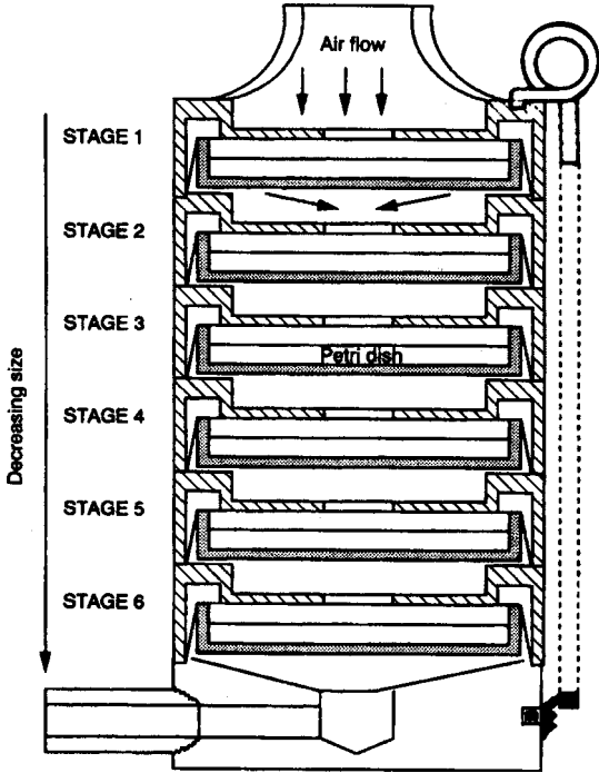
Figure 14.3 Sieve-type sampler (Andersen sampler) for biological aerosols.
