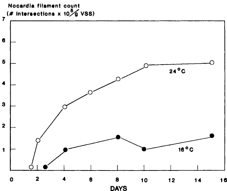
Figure 9.20 Effect of MCRT and temperature on Nocardia populations in bench-scale activated sludge units. From Cha et al. (1992). (Courtesy of Water Environment Federation.)
