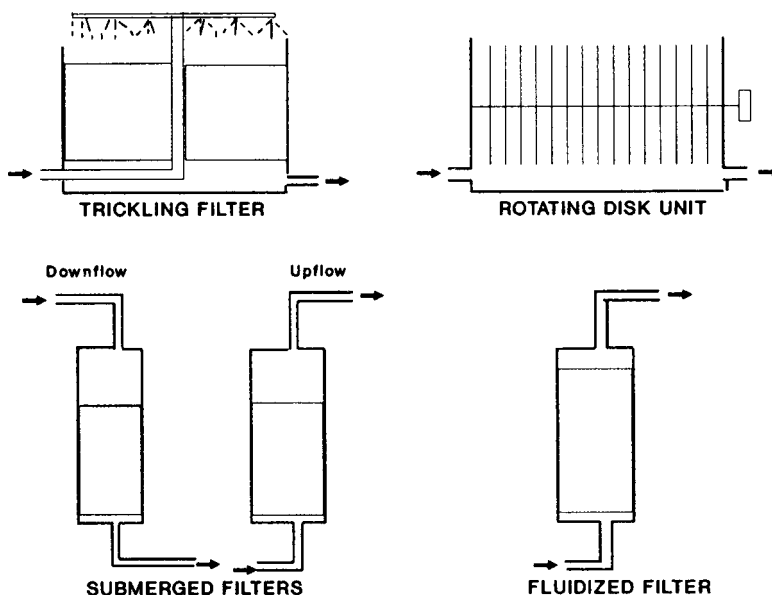
Figure 10.1 Biofilm reactors used for wastewater treatment. Adapted from Harremoës (1978).
