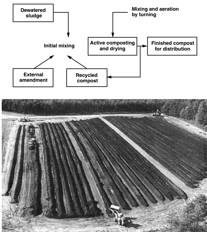
Figure 12.4 Composting. Conventional windrow process. From Benedict et al. (1988). (Courtesy of Noyes Data Corp. and W. D. Burge.)
