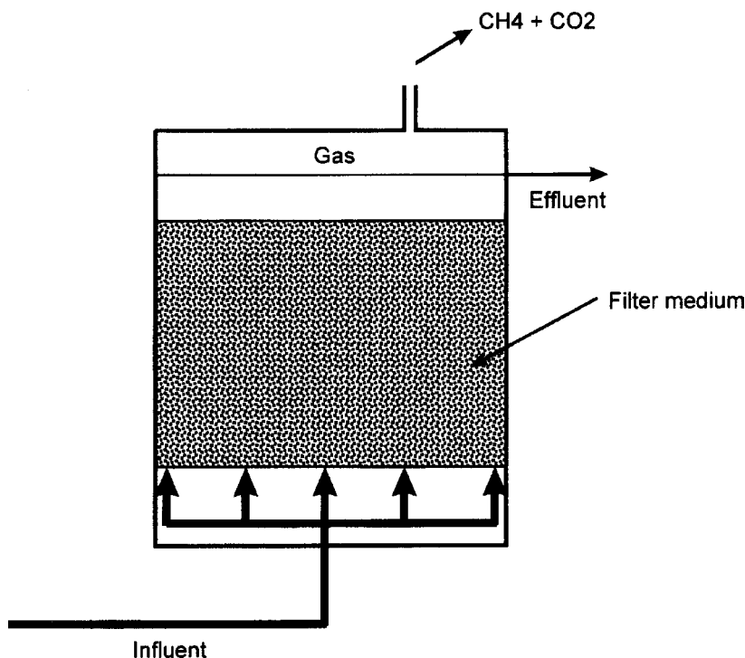
Figure 13.11 Anaerobic filter. From Jewell (1987). (Courtesy of the American Chemical Society.)
