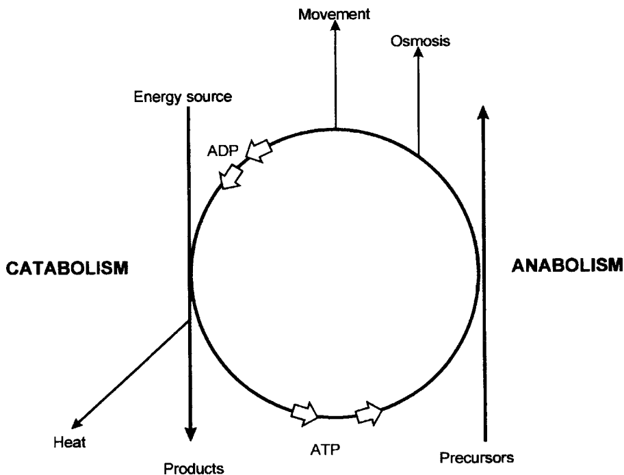
Figure 2.3 Relationship between anabolic and catabolic reactions. From Scragg (1988).
