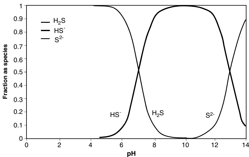
Figure 14.9 \text{H}_2\text{S} dissociation.
