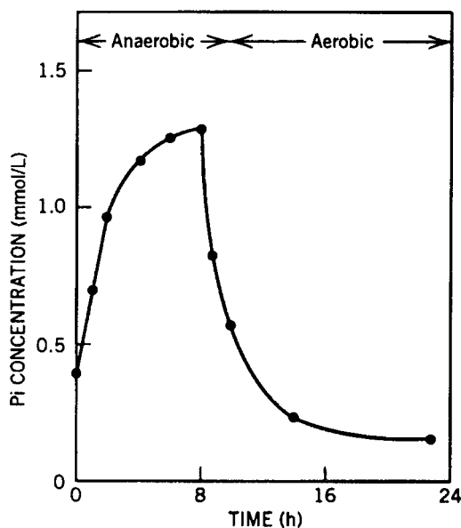
Figure 3.4 \text{P}_i release and uptake by a laboratory anaerobic–aerobic activated sludge. From Hiraishi et al. (1989).
