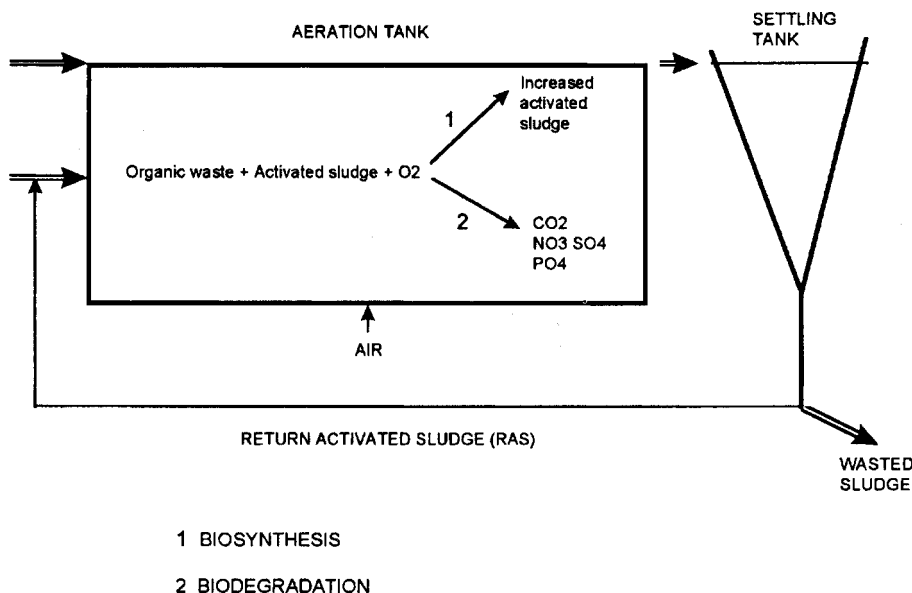
Figure 8.14 Organic matter removal by the activated sludge process. Adapted from Curds and Hawkes (1983).
