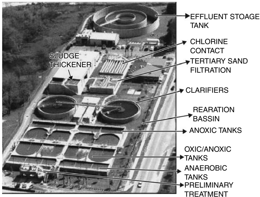
Figure 8.26 Aerial view of the University of Florida water reclamation plant.
