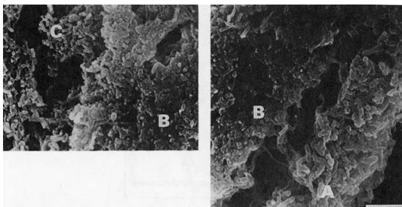
Figure 13.10 Three-layered structure of a sludge anaerobic granule (bar = 5 µm): A, exterior heterogeneous layer with rods, filaments, and cocci; B, second layer containing predominantly rods and cocci; C, homogenous core containing a large number of cavities, surrounded by one bacterial morphology. From MacLeod et al. (1990). (Courtesy of American Society of Microbiology and S. Guiot.)
