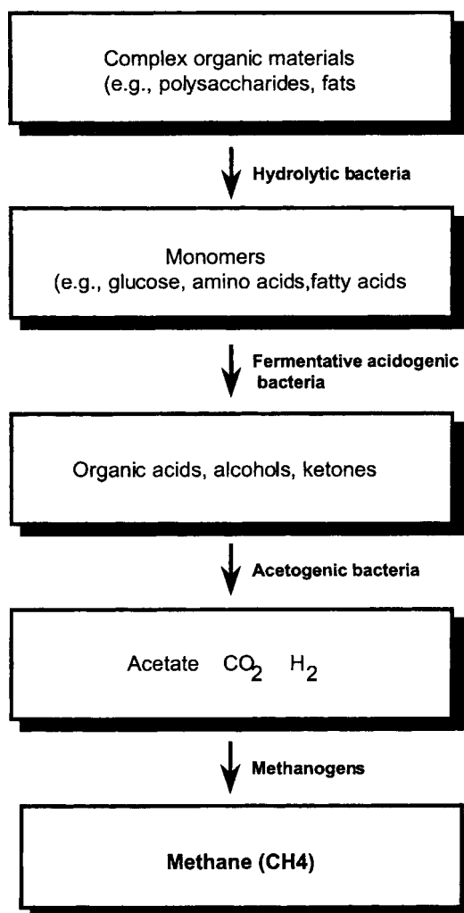
Figure 13.4 Metabolic bacterial groups involved in anaerobic digestion of wastes.
