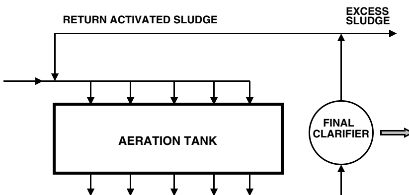
Figure 8.20 Nitrification systems. From U.S. EPA (1977).
