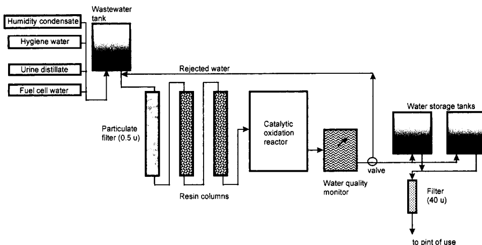
Figure 23.9 Wastewater treatment on board the International Space Station. Adapted from Hurst et al. (1998).
