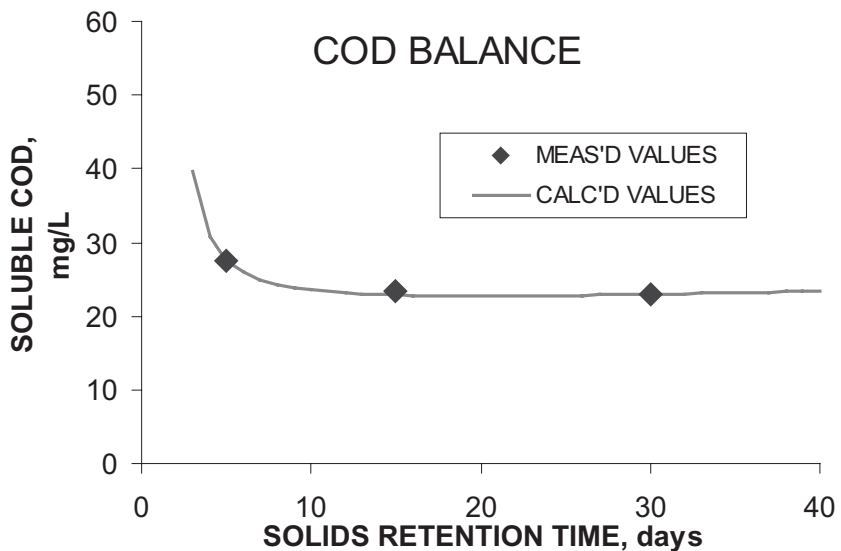
FIGURE 5.3 Example of modeling effluent chemical oxygen demand versus solids retention time using eq 5.4 (Young and Cowan, 2004; used with permission).
