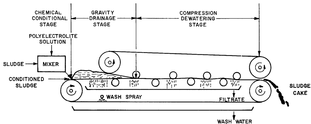
FIGURE 9.21 A schematic of a belt filter press.
