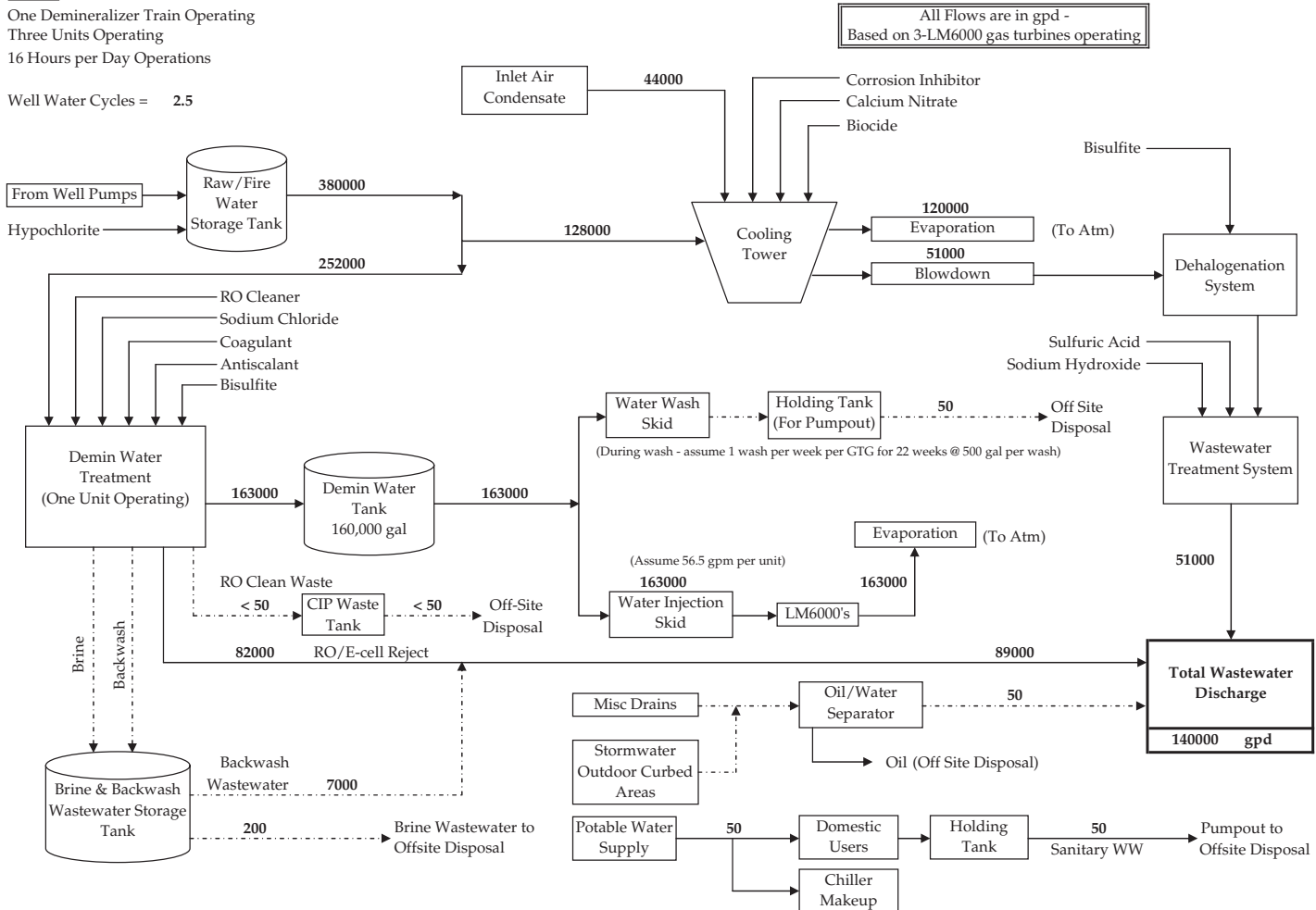
FIGURE 4.1 Mass balance for a combined cycle power-generating station (gpd \times 0.003785 = \text{m}^3/\text{d} ; gpm \times 5.451 = \text{m}^3/\text{d} ).
