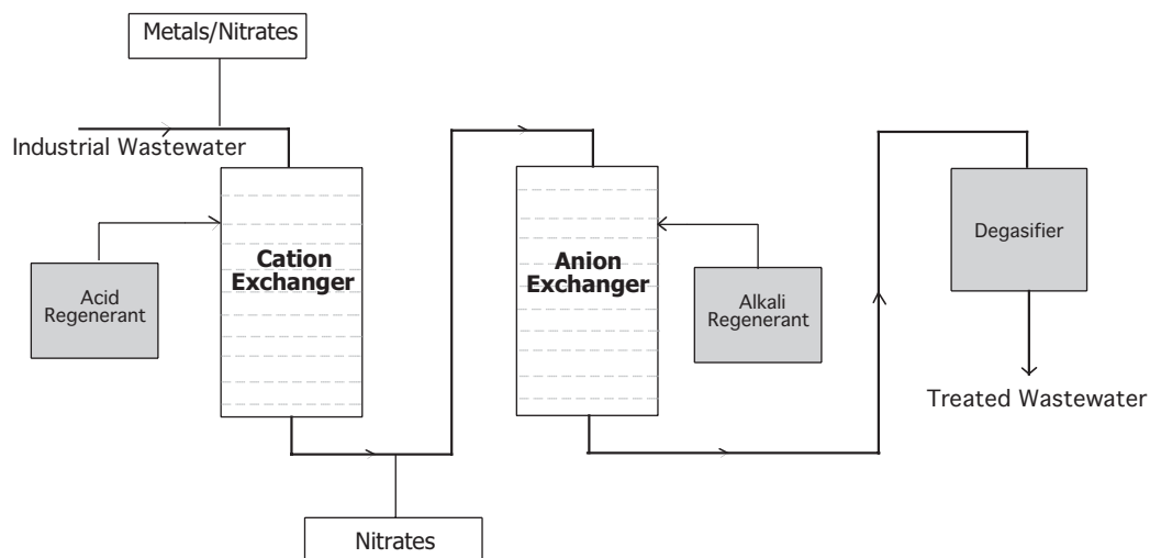
FIGURE 12.5 A process diagram of a typical ion-exchange system.
