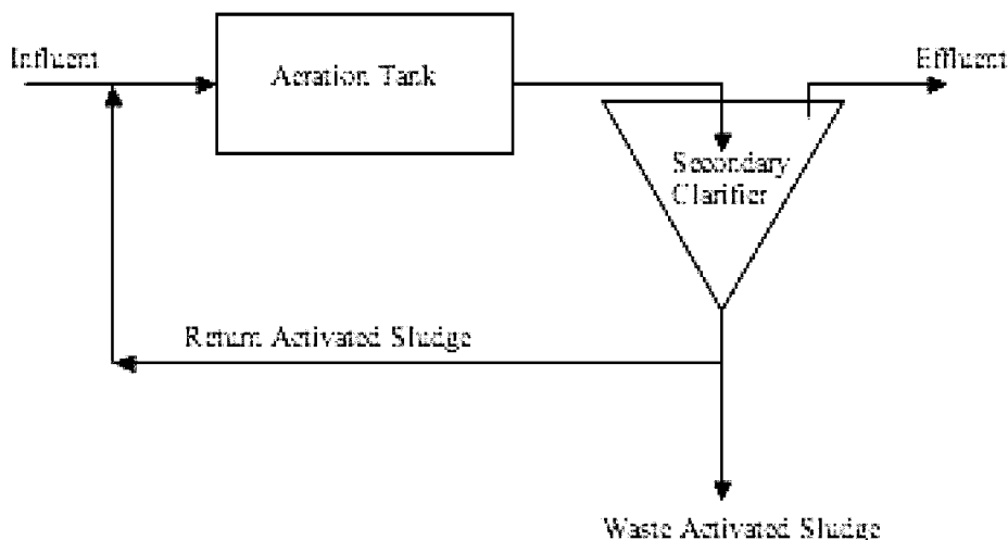
FIGURE 13.2 A schematic of the activated sludge process.
