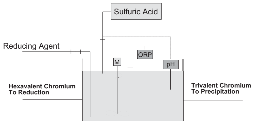
FIGURE 12.6 A schematic of a typical hexavalent chrome reduction system.
