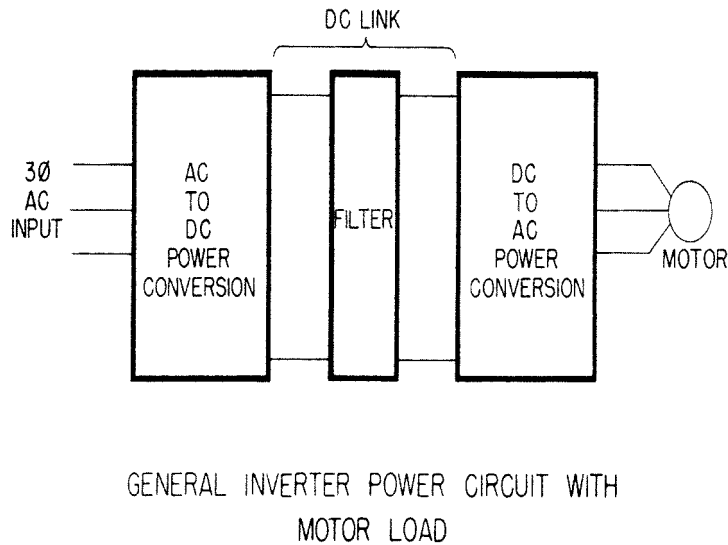
FIGURE 14.17 A schematic of a variable-frequency controller (courtesy of Siemens Energy & Automation, Inc., Alpharetta, Georgia).
