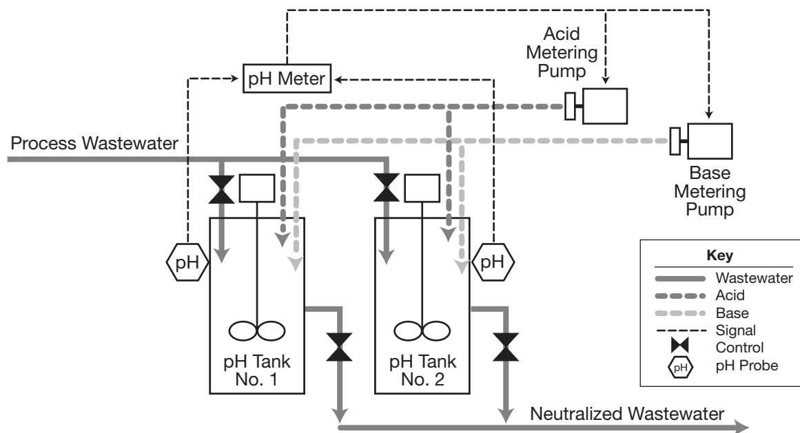
FIGURE 11.2 A batch pH control system schematic.
