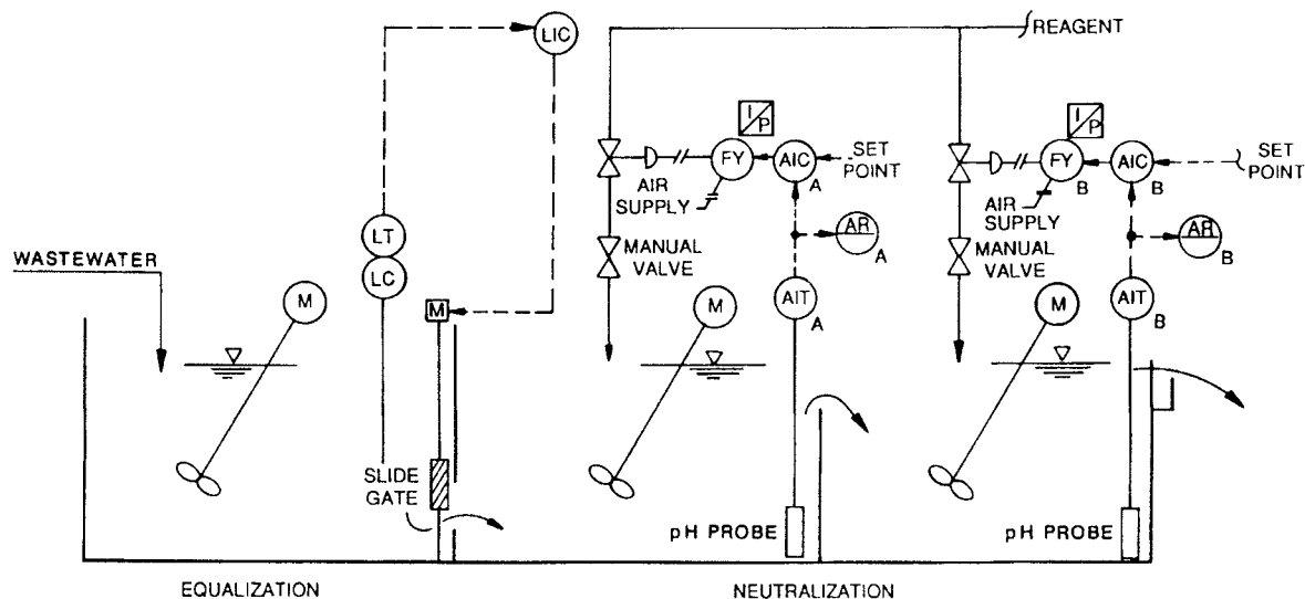
FIGURE 14.24 A process diagram of a two-stage neutralization system with equalization.
