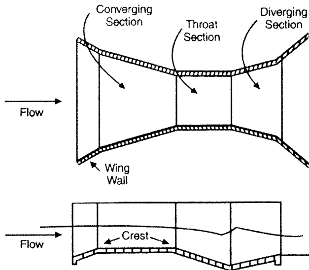
FIGURE 14.2 A schematic of a Parshall flume.
