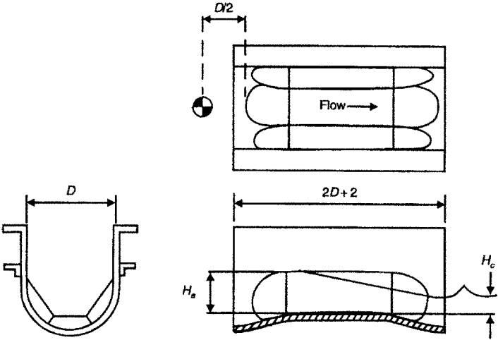
FIGURE 14.3 A schematic of a Palmer-Bowlus flume (courtesy of Free Flow, Inc., Omaha, Nebraska).
