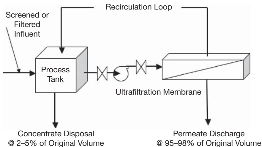
FIGURE 10.6 A schematic of an ultrafiltration process.
