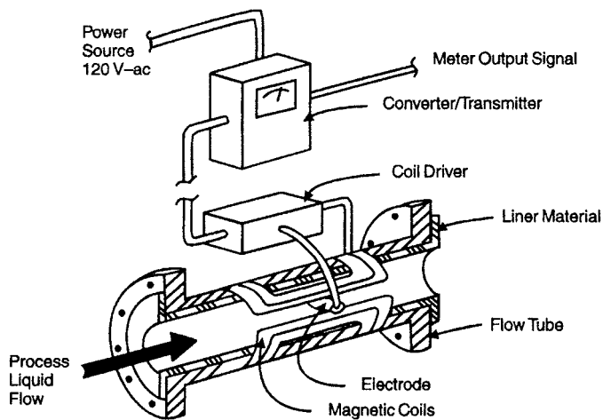
FIGURE 14.7 A schematic of a magnetic flow meter.
