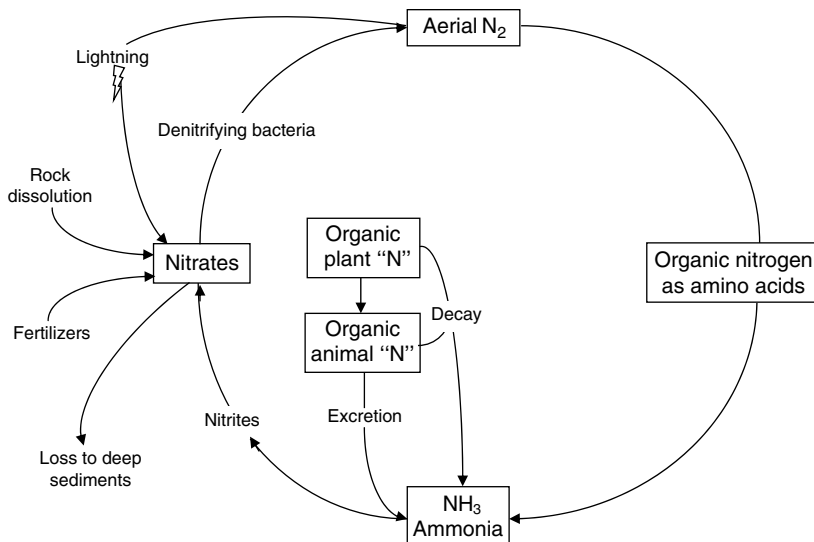
FIGURE 6.5 Nitrogen cycle.
