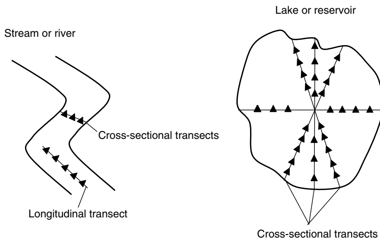
FIGURE 8.1 Transect sampling.
