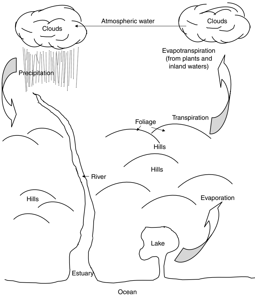
FIGURE 2.2 Water cycle.
