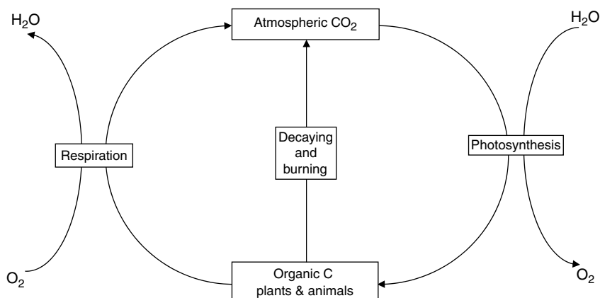
FIGURE 6.4 Carbon cycle.
