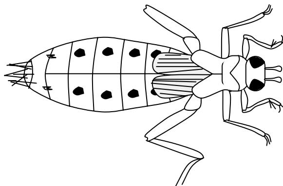
FIGURE 6.31 Dragonfly nymph.
