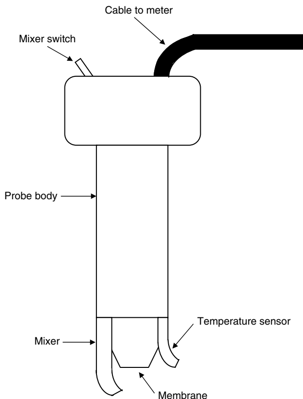
FIGURE 8.15 Dissolved oxygen-lab probe.
