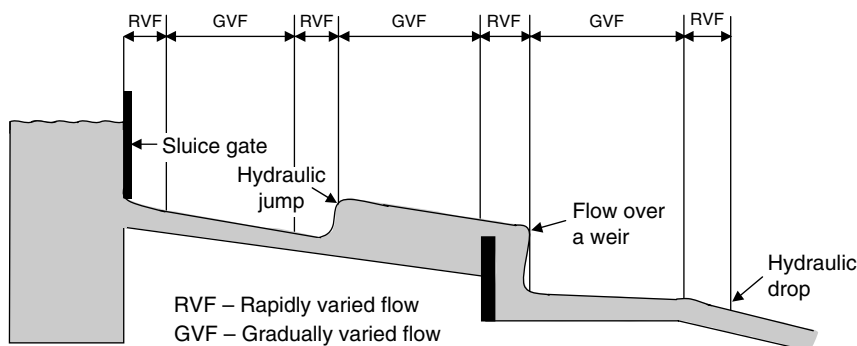
FIGURE 3.16 Varied flow.
