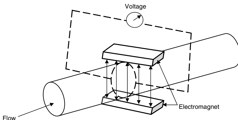
FIGURE 3.28 Magnetic flowmeter.
