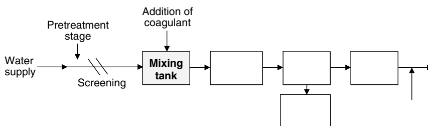
FIGURE 9.3 Coagulation.
