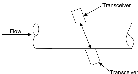
FIGURE 3.30 Time-of-flight ultrasonic flowmeter.
