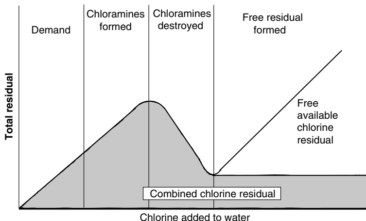
FIGURE 9.9 Breakpoint chlorination curve.
