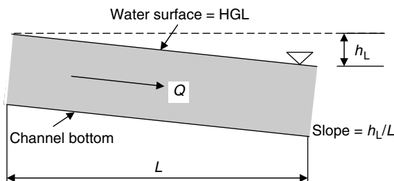
FIGURE 3.21 Steady uniform open-channel flow—where the slope of the water surface (or HGL) is equal to the slope of the channel bottom.
