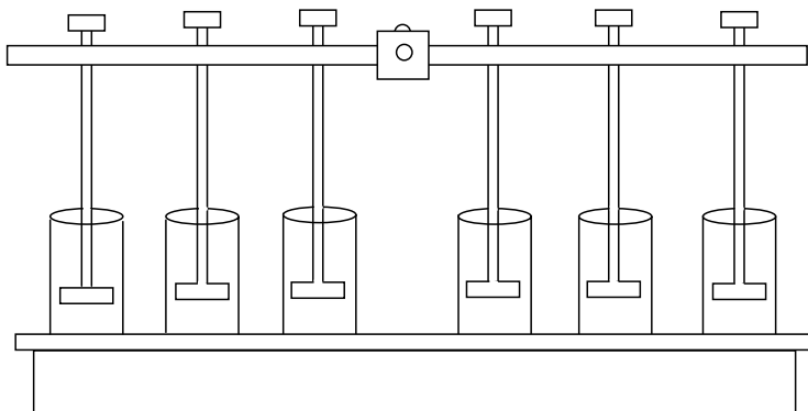
FIGURE 9.4 Variable speed paddle mixer used in jar testing procedure.
