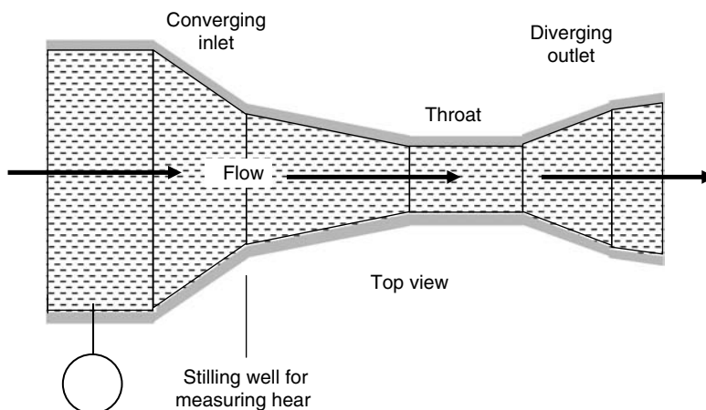
FIGURE 3.36 Parshall flume.
