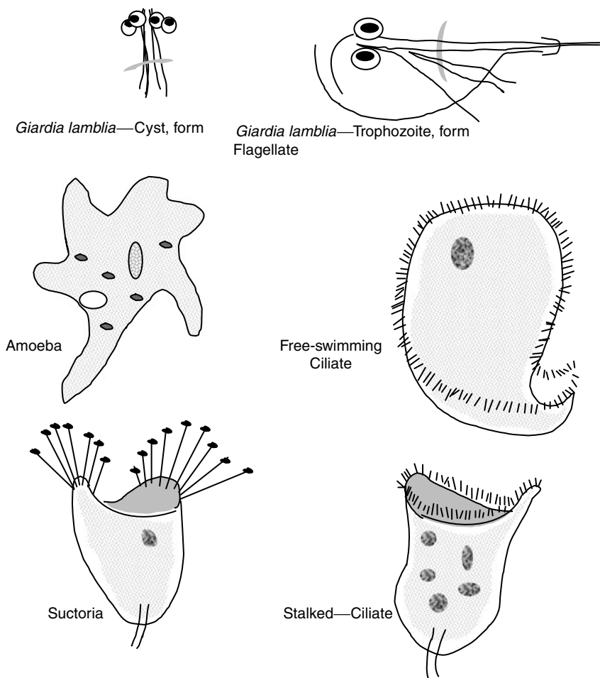
FIGURE 5.5 Protozoa.
