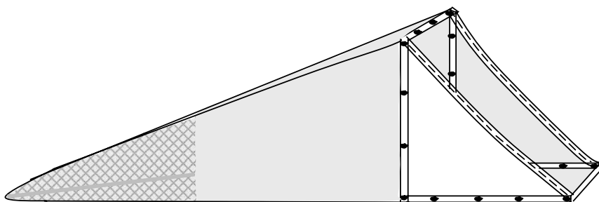
FIGURE 8.8 Surber sampler.
