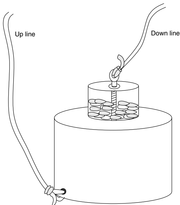
FIGURE 8.9 Homemade dredge.
