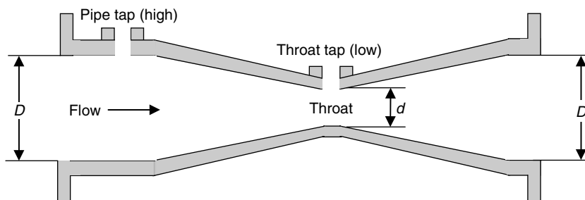
FIGURE 3.25 Venturi tube.
