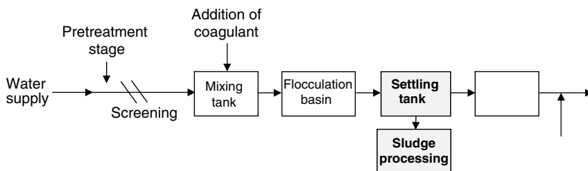
FIGURE 9.6 Sedimentation.
