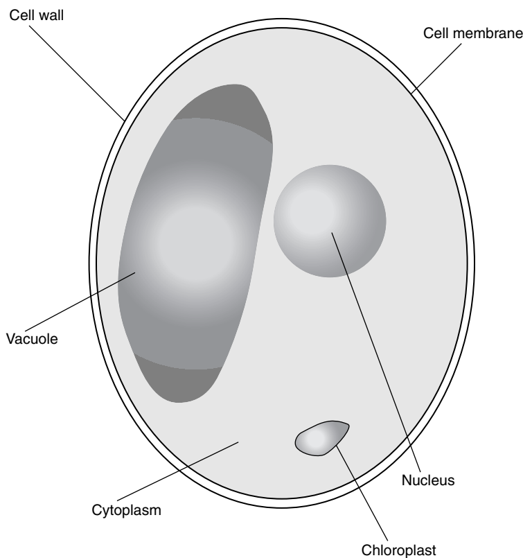
FIGURE 5.1 Plant cell.
