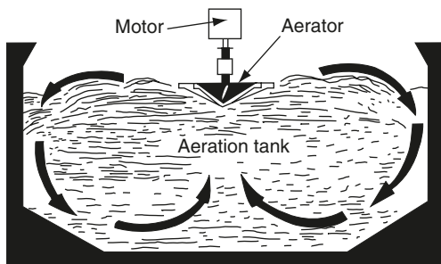
Figure C.6 Cone aerator.
