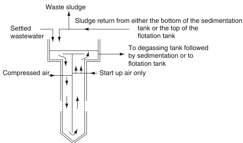
Figure D.1 Deep shaft process.
