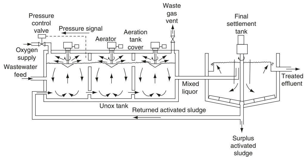
Figure O.5 Oxygen activated sludge, Unox system.
