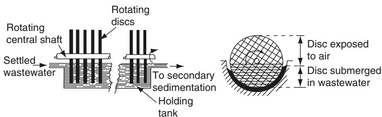
Figure R.10 Rotating biological contactor.
