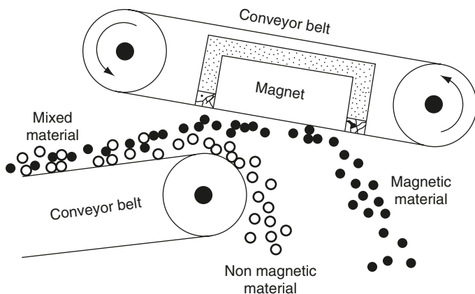
Figure O.3 Overband magnetic separator.
