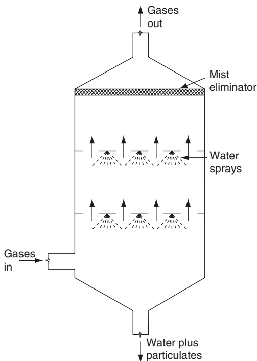
Figure S.13 Gravitational spray chamber.
