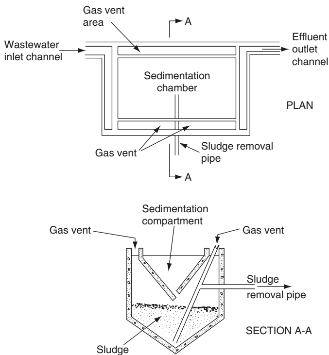
Figure I.1 Imhoff tank.
