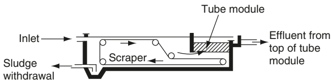
Figure I.3 Inclined tube settling module in horizontal flow sedimentation tank.
