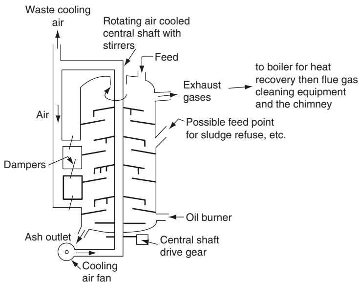
Figure M.7 Multiple hearth incinerator.
