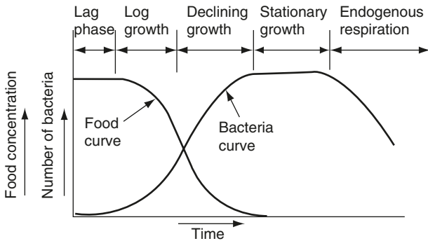
Figure M.2 Microbial growth curve.
