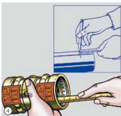
Se marchează adîncimea de introducere. \varnothing 64,0 \text{ mm} = 43 \text{ mm} \varnothing 76,1 \text{ mm} = 50 \text{ mm} \varnothing 88,9 \text{ mm} = 50 \text{ mm} \varnothing 108,0 \text{ mm} = 60 \text{ mm}
