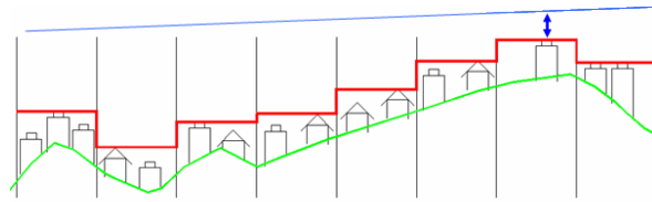
Figure 1. 5 Principle of taking into account height of construction development in assessing pressure ratios in water mains network
