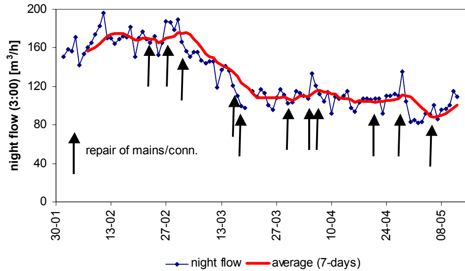
Figure 21. Long term overnight flow trend (DMA 'S')
