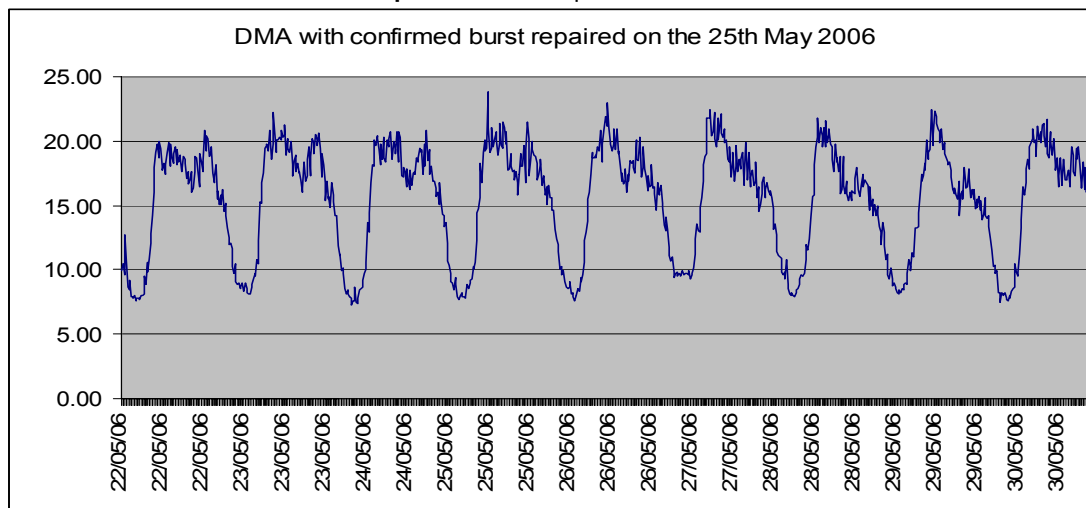
Graph 1.3 – Burst repaired 25/05/2006
