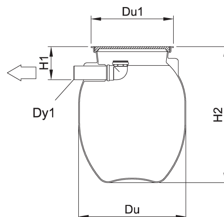
рис. 4.5 б (HEK 120 LK)
