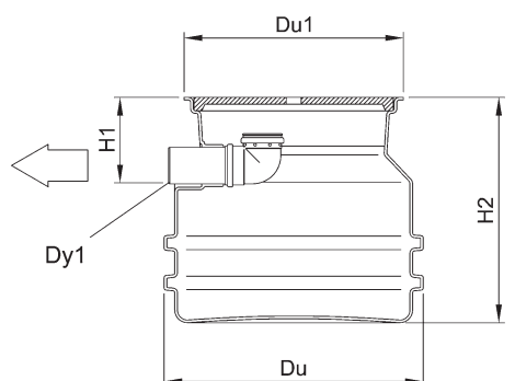
рис. 4.5 а (HEK 40 LK)
