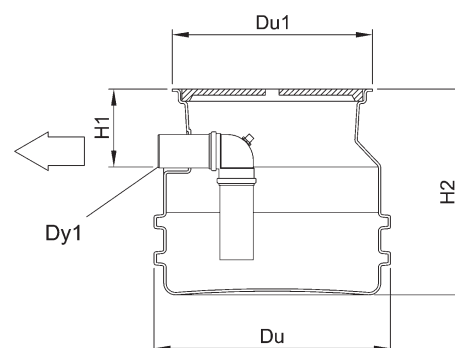
рис. 4.5 б (HEK 120 LK)
