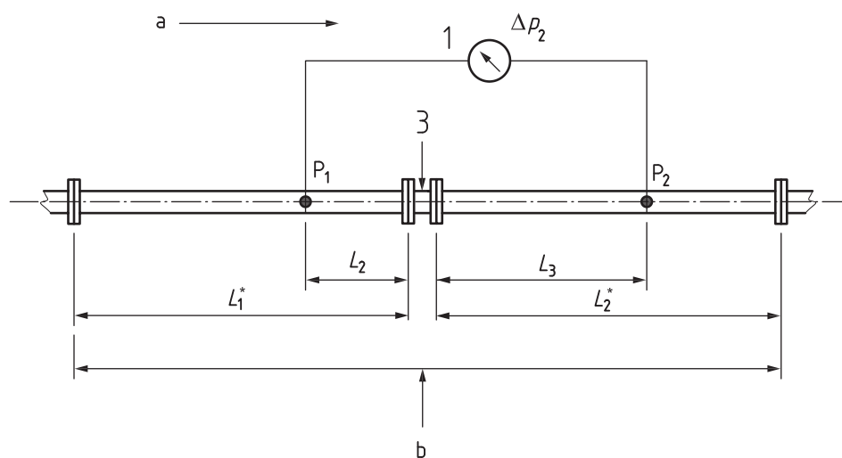
b) (Pipe and water meter) pressure loss
