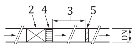
Test 4A: with a straightener
