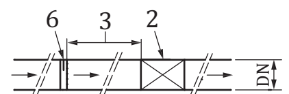
Test 5: without a straightener
