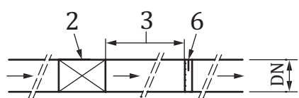
Test 6: without a straightener
