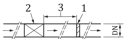
Test 2: without a straightener
