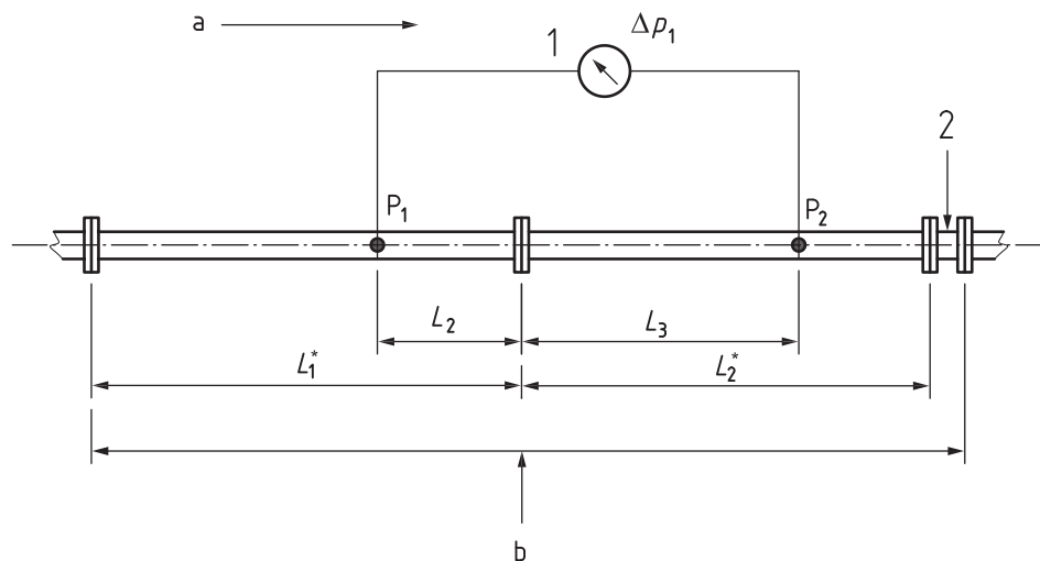
a) Pipe pressure loss
