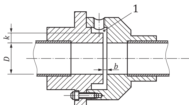
Figure H.1 — Example of drilled hole type of pressure tapping with ring chamber, suitable for small/medium diameter test sections
