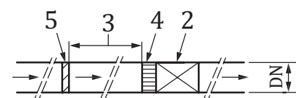
Test 3A: with a straightener
