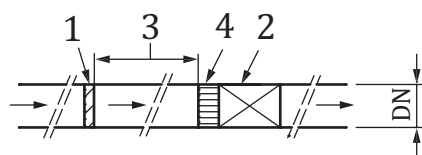
Test 1A: with a straightener
