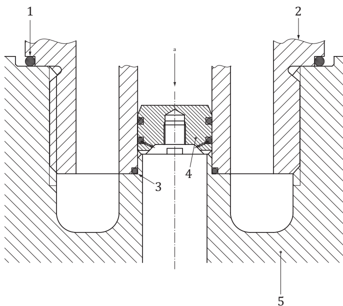
Figure E.2 — Example of a manifold for pressure testing concentric meter seals
